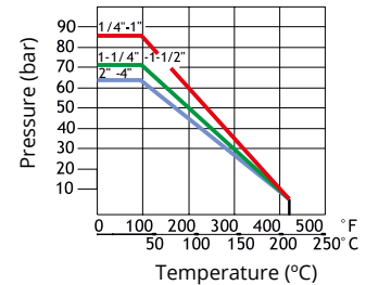
Pressure-Temperature Diagram
