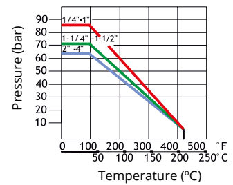
Pressure-Temperature Diagram
