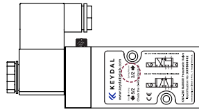
3/2 Tip Ayarlı Solenoid Valf
